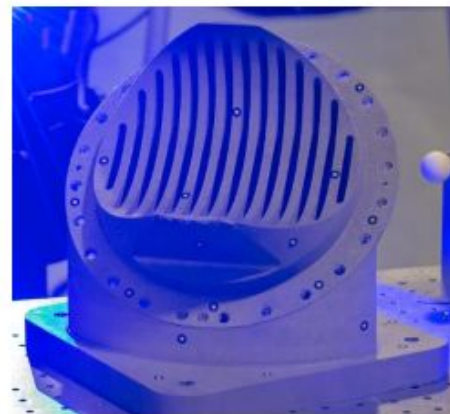
(c) NASA engine baffle [3]
